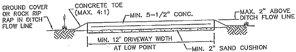
SECTION B-B
